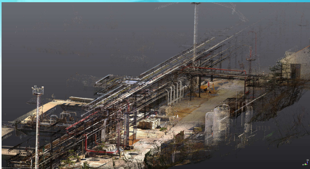
6 Cjevni most - Point Cloud
