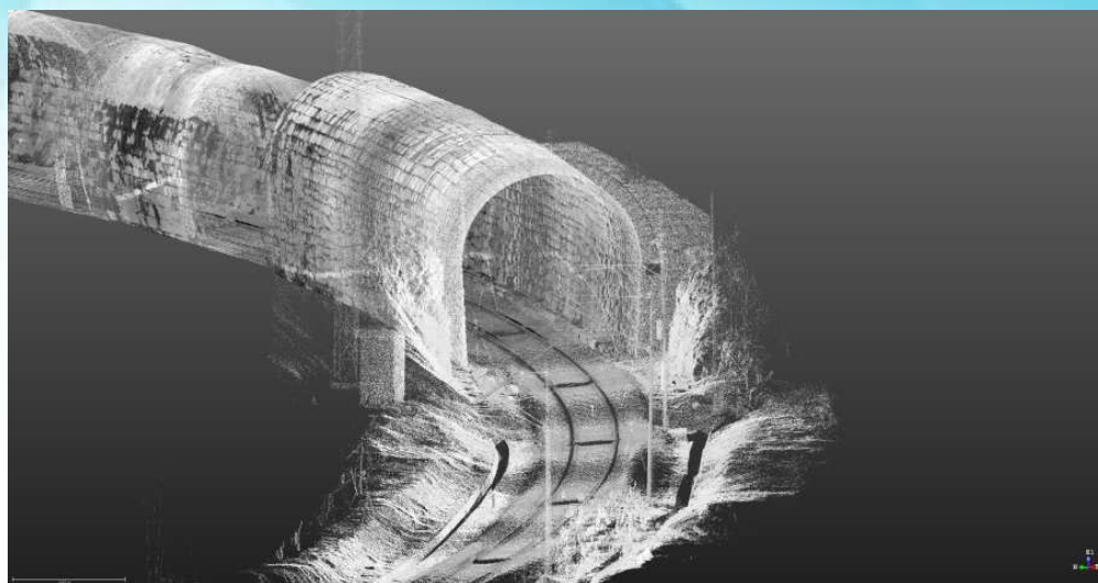
9 Oblak točaka - Tunnel
